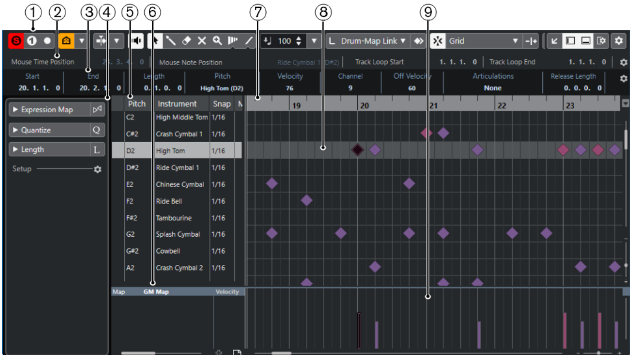
The Drum Editor in the lower zone of the Project window:
